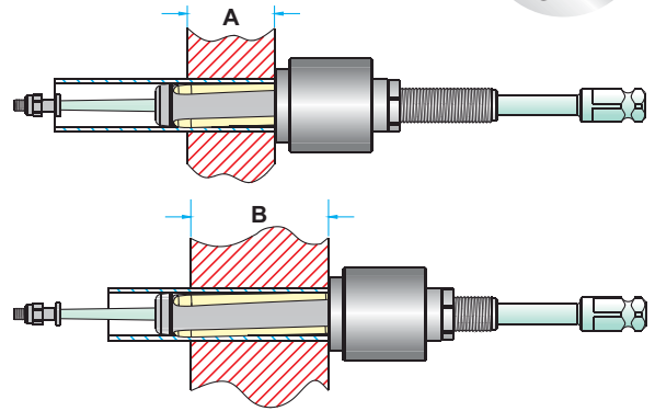
FORTUBES INTERNAL DIAMETER FROM (8.4 mm) .334" TO (36.3 mm) 1.43"
